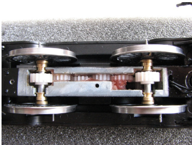
Assembled wheels installed in the chassis.
