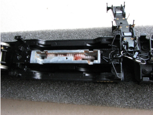
Keeper plate removed with wheel sets removed.
