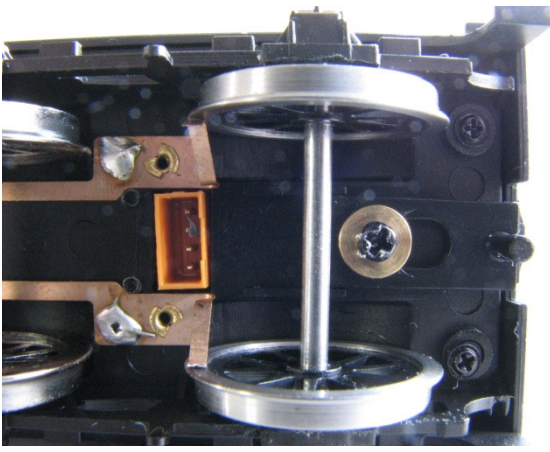
Another view of modified pickups.
