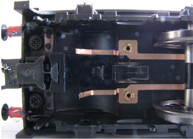
Bachmann pickups with wheels removed.
